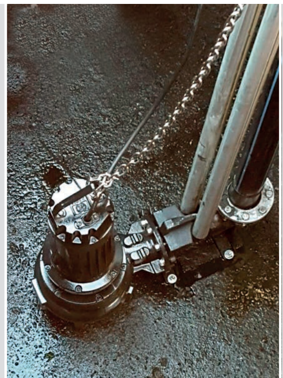
Lifting station pumping rainwater from collection tanks (Italy) Four ZUG V 100B 5.5/4 AW pumps
